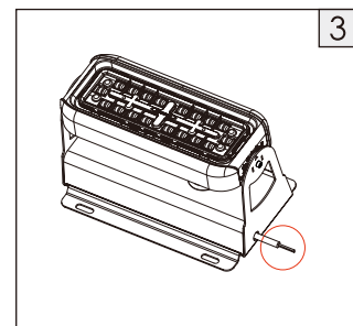
3. Connect to the L, N, and G wires of AC input correctly.
