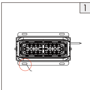
1. Mount the luminaire onto the wall with four screws. (recommend M8 screws)
