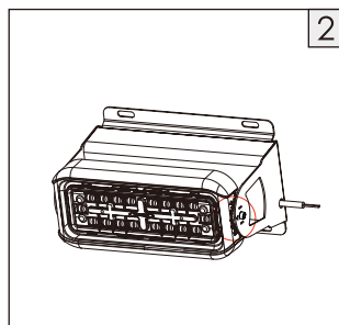
2. Loosen the M6 screws at sides to adjust the fixture to a right angle. Then tighten up the screws.
