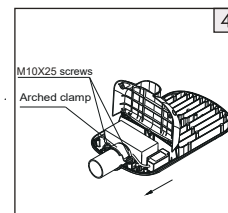
4. Stick the pole arm under the arched clamp and tighten up the screws.
