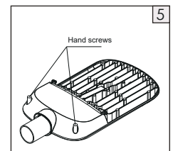
5. Close the cover and tighten up the hand screws.
