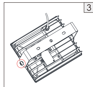
3. Loosen the M10 screws on brackets to adjust to a proper angle.
