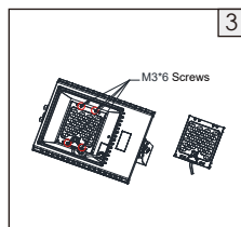
3. Undo the four M3x6 cross recessed pan head screws on the module, and take it out.
