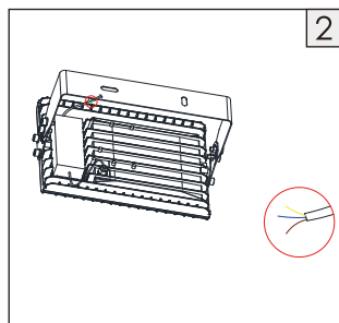
2. Connect the wires to AC input. Make sure it grounded sufficiently.
