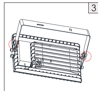
3. Loosen the M8x20 screws on brackets to adjust to a proper angle.
