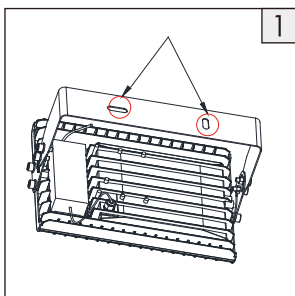
1. Fixate the luminaire onto the mounting surface with screws (recommend M10 screws).
