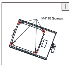
1. Undo the four M4x10 hex socket head cap screws to remove the glass.
